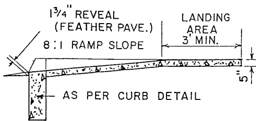
SECTION B-B
