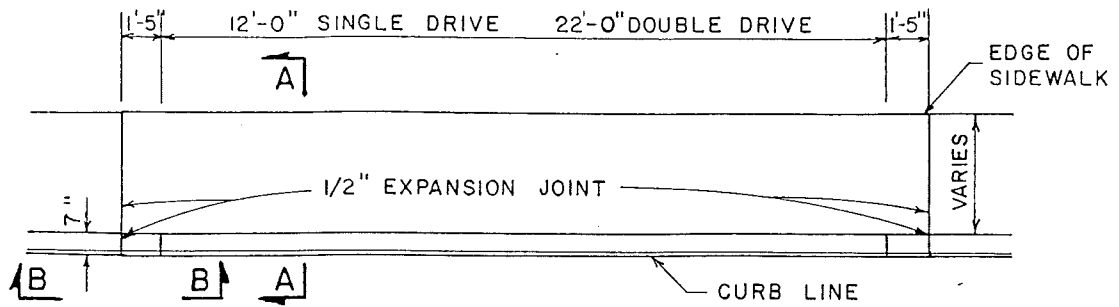
PLAN - DEPRESSED CURB DRIVE ENTRANCE
