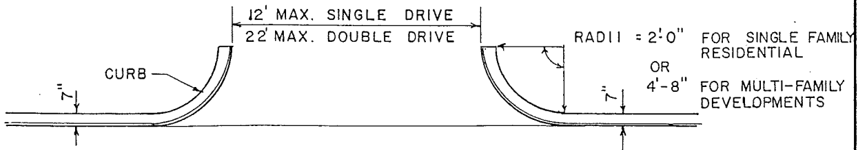
PLAN - DRIVEWAY ENTRANCE
